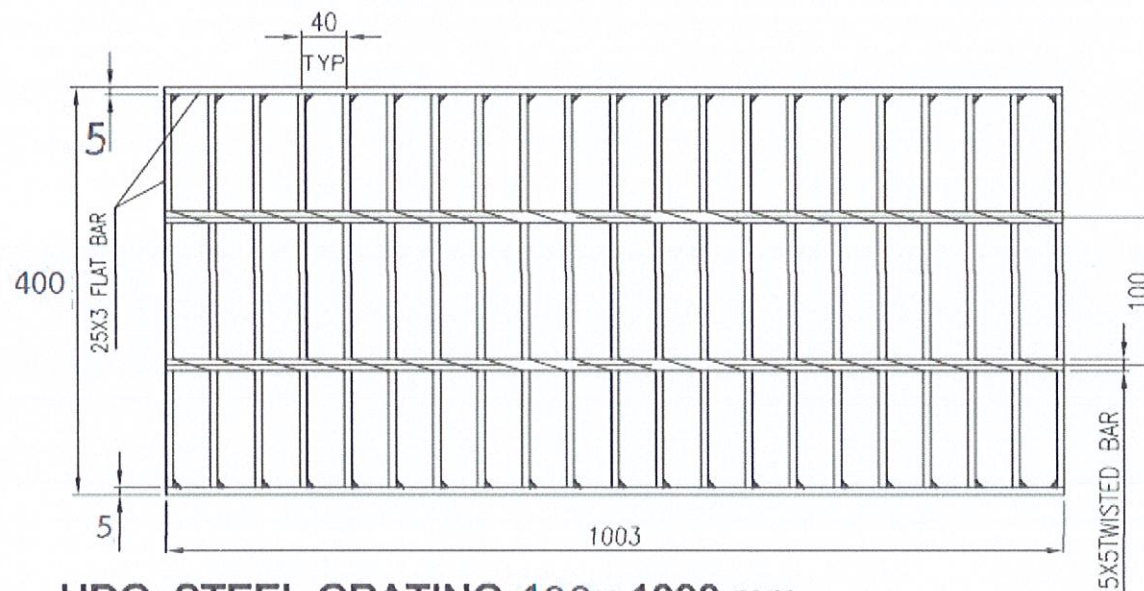
HDG. STEEL GRATING 400x 1000 mm.
